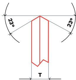
K PROFILED GRINDING WHEEL
