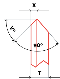
N PROFILED GRINDING WHEEL
