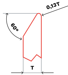
D PROFILED GRINDING WHEEL
