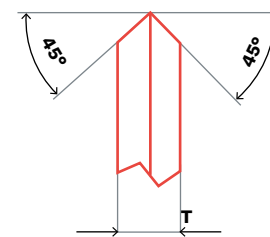
P PROFILED GRINDING WHEEL
