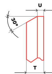
M PROFILED GRINDING WHEEL
