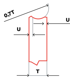
J PROFILED GRINDING WHEEL
