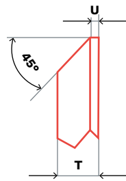
C PROFILED GRINDING WHEEL
