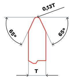
M PROFILED GRINDING WHEEL
