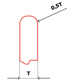
F PROFILED GRINDING WHEEL
