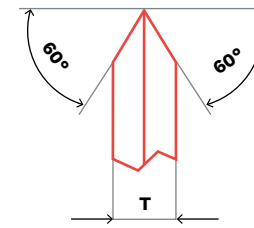
I PROFILED GRINDING WHEEL
