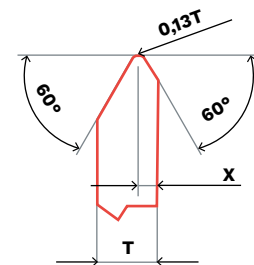
P PROFILED GRINDING WHEEL
